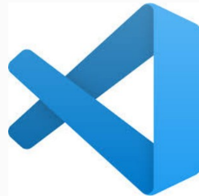
VScode
